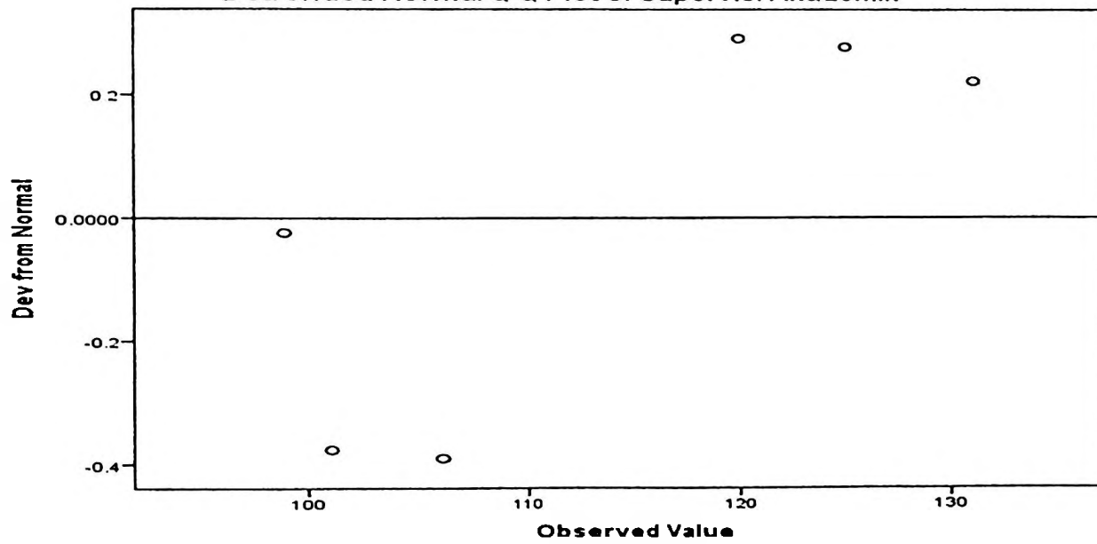
Detrended Normal Q-Q Plot of Supervisi Akademik
