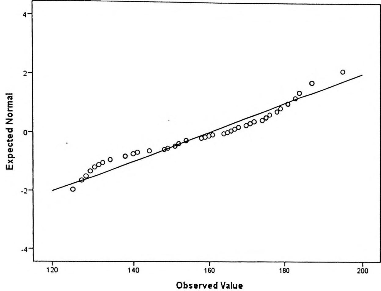
Normal Q-Q Plot of Kompetensi Guru PAK
