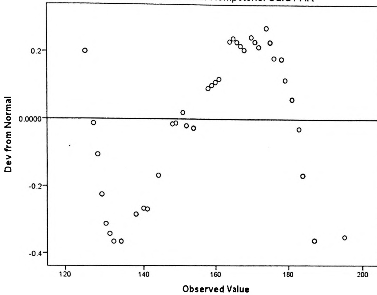
Detrended Normal Q-Q Plot of Kompetensi Guru PAK
