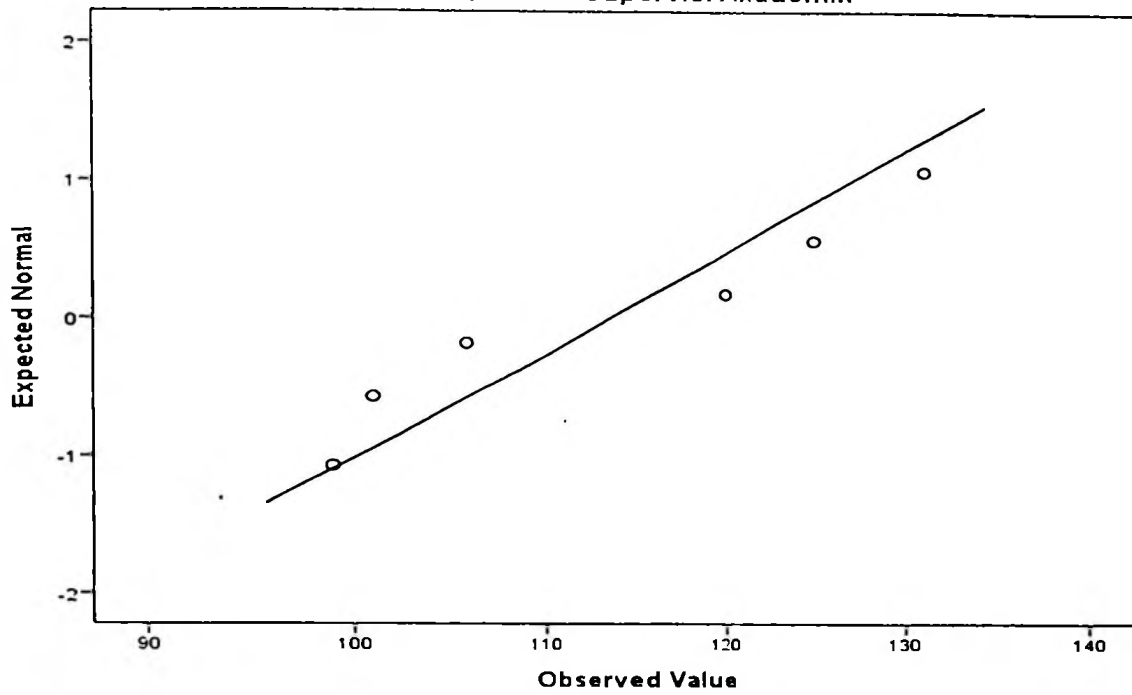
Normal Q-Q Plot of Supervisi Akademik
